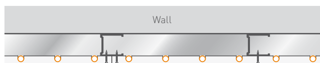
▲ Section through a CW/UW profile metal substructure, without cavity insulation.
