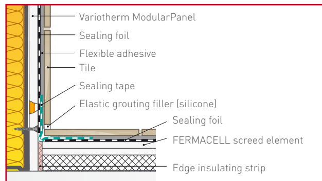
▲ Wall-screed structure in areas subjected to water loads
