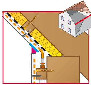
▲ Pitched roof to jamb wall
