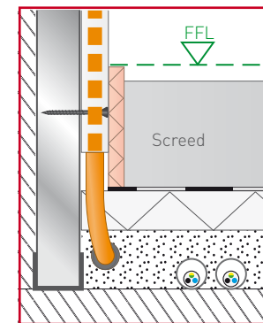
▲ Example of finished press-fit coupling in floor construction (new building)
