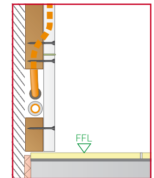
▲ Example of finished press-fit coupling with existing floor (rehabilitation)
